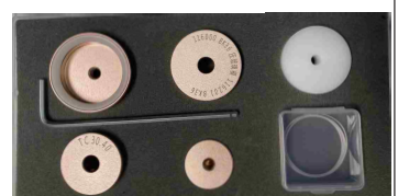
ST-5446-Die set use to replace crystals & gaskets for RLX. Made for 116000 BK36
